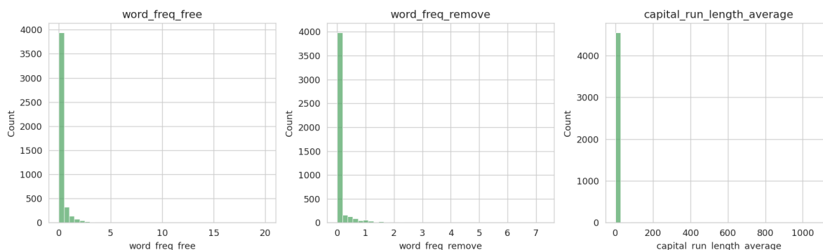
Figure 3: Distribution of three representative features: word_freq_free , word_freq_remove , and capital_run_length_average .
