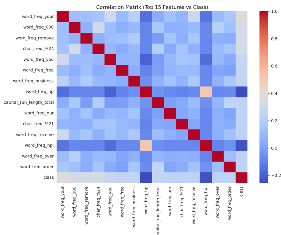
Figure 2: Correlation heatmap of the 15 features most correlated with the target class, along with the class label.
