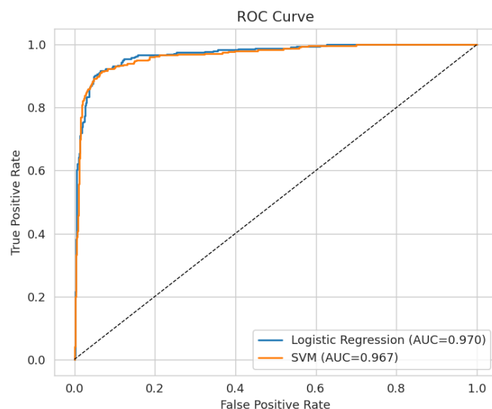
Figure 6: ROC curves for Logistic Regression and SVM on the test set.
