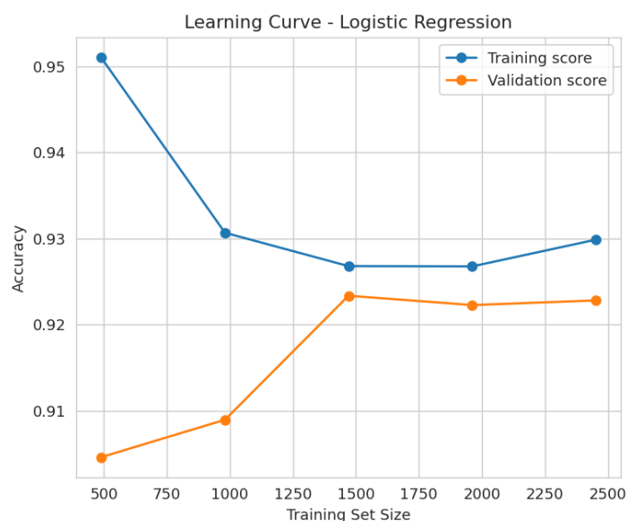
Figure 8: Learning curve for the tuned Logistic Regression model.
