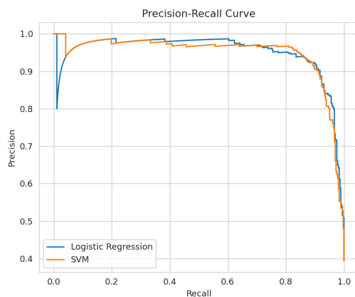
Figure 7: Precision-Recall curves for Logistic Regression and SVM on the test set.
