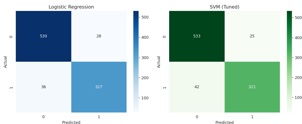
Figure 5: Confusion matrices for the tuned Logistic Regression (left) and tuned SVM (right) on the test set.
